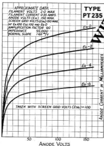
Characteristic Curves of Average PT 235 Valve.
