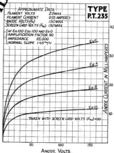
Characteristic Curves of Average PT 235 Valve.
